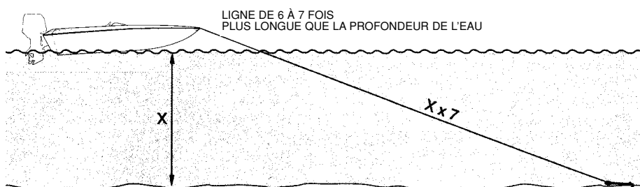
FIGURE 7-4 ANCRAGE
