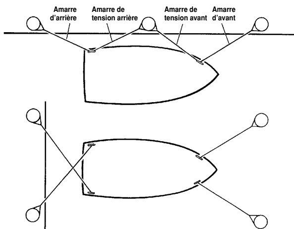
FIGURE 7-6 AMARRES
