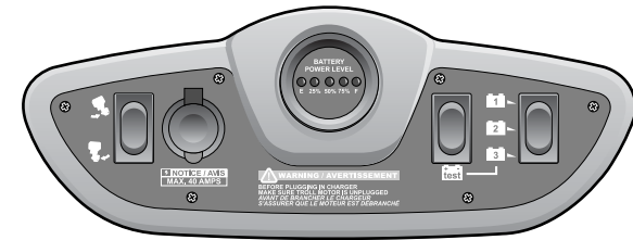
FIGURE 4-5 12, 24 OR 36 VOLT BOW TROLLING PANEL
