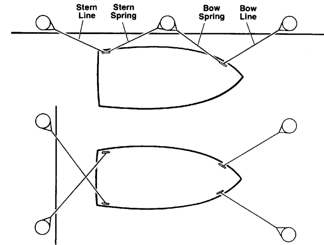
FIGURE 7-6 MOORING LINES
