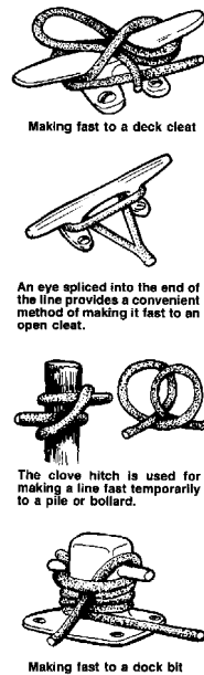
FIGURE 7-5 MOORING LINE TIES
